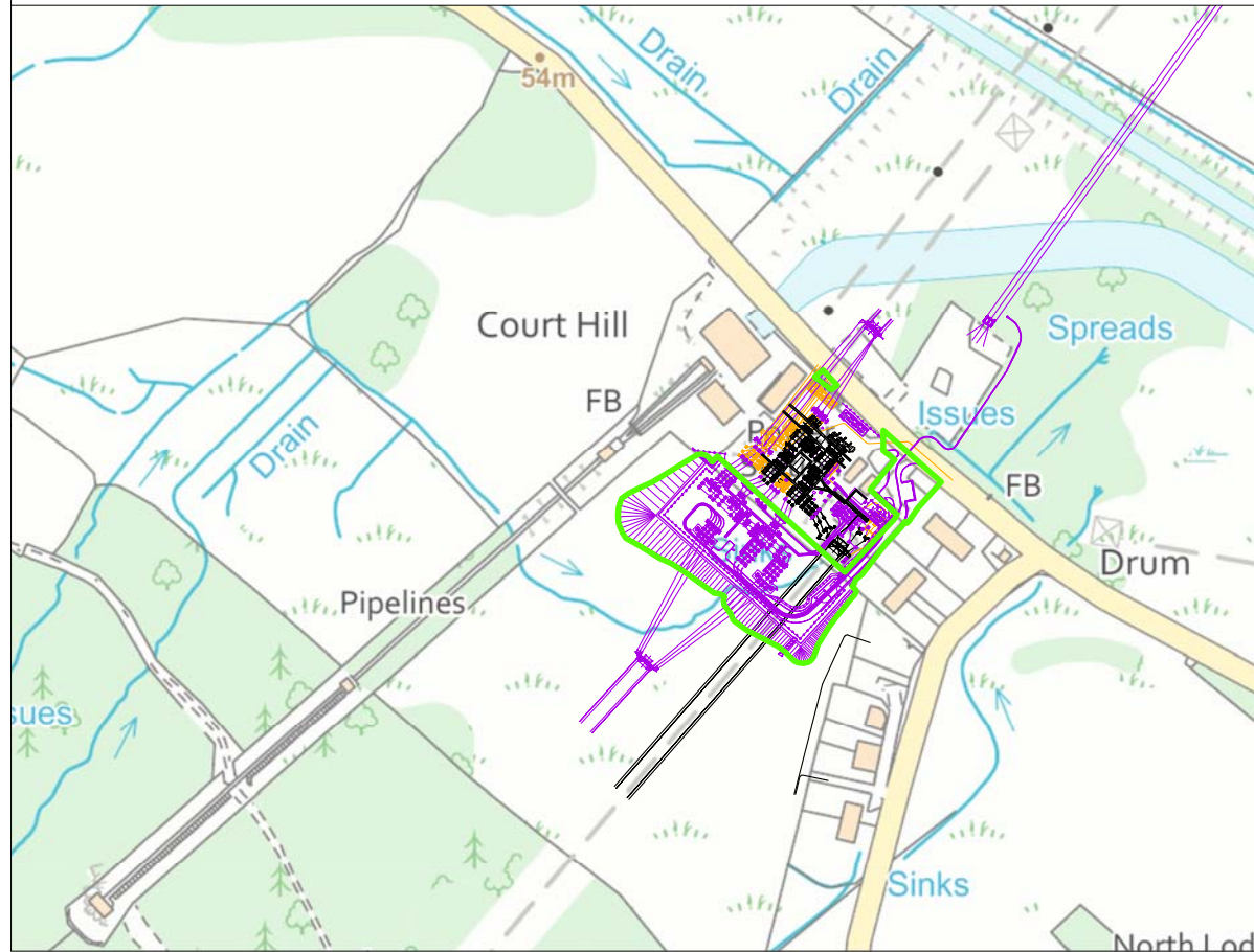
Option 3: move entire substation (proposed and existing) to the opposite side of Glenlee Power Station as an air insulated substation
