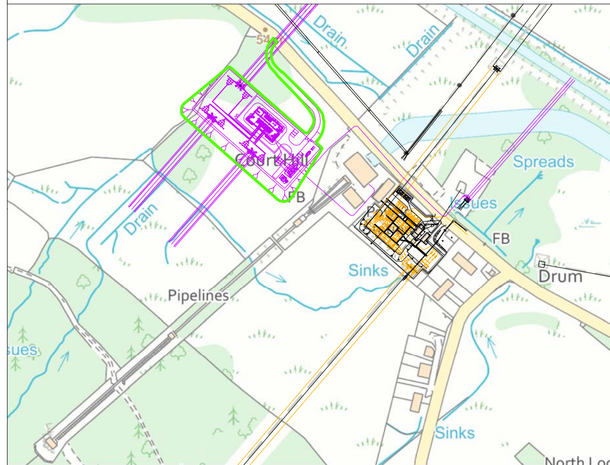
Option 4: move entire substation (proposed and existing) to the opposite side of Glenlee Power Station as a gas insulated substation
